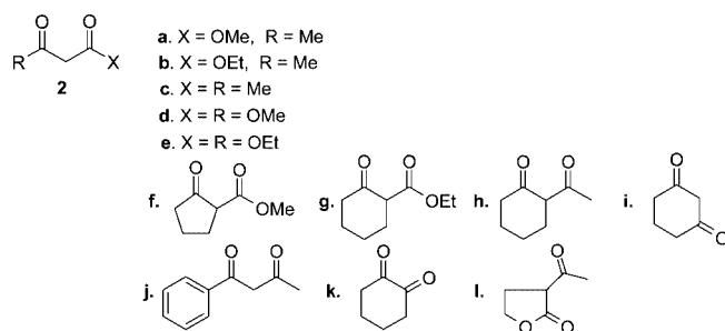
Figure 2. Michael donors 2 used in conjugate-addition and CAIRC reactions.
