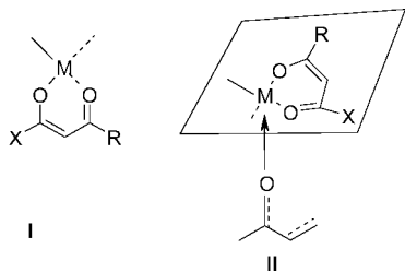
Figure 3. Possible structures of metal enolate intermediates.
