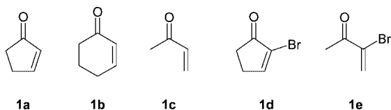
Figure 1. \alpha,\beta -Unsaturated ketones 1a–1e used as Michael acceptors.
